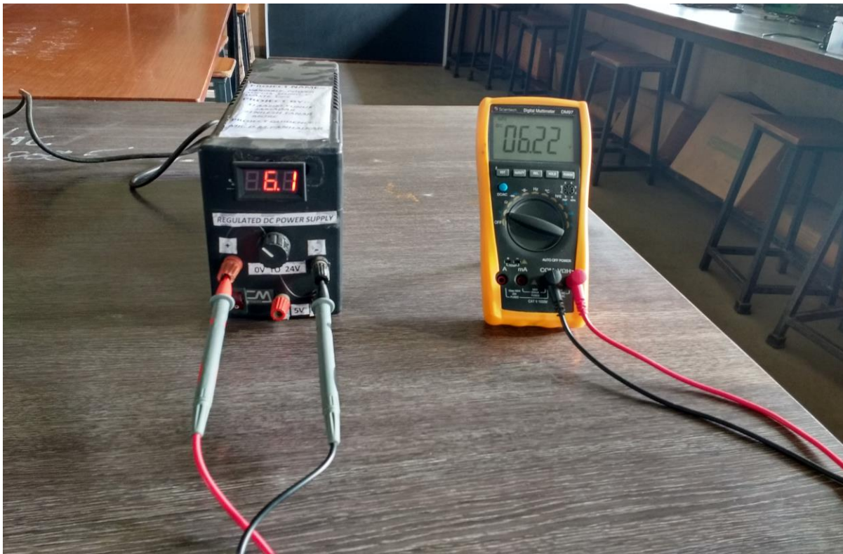
Photo: Developed D.C. Power Supply by electronics faculty and B.SC. III students
