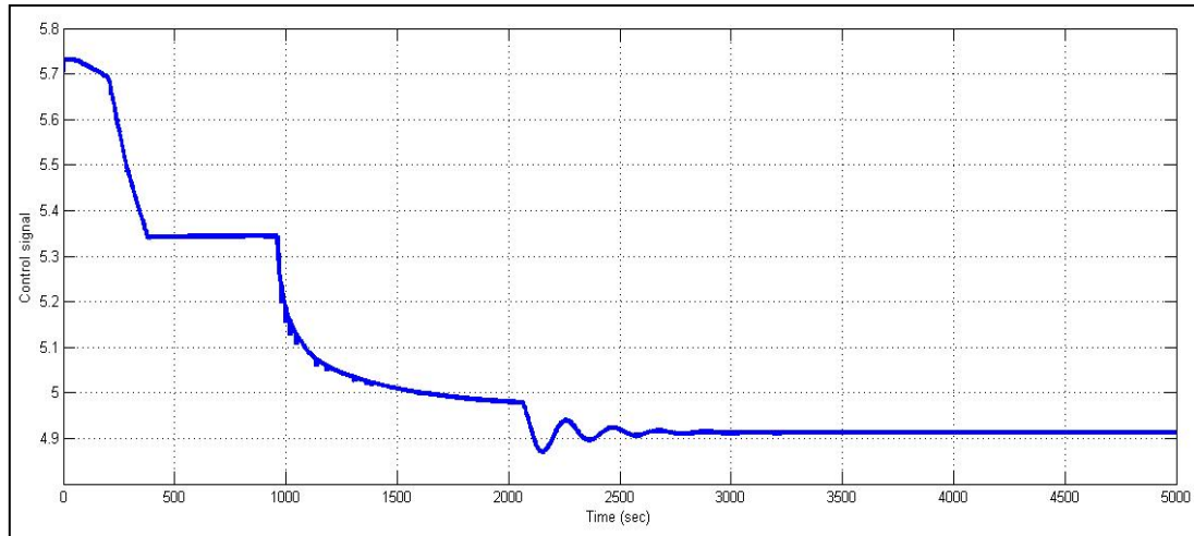
Figure 12. Control Signal
