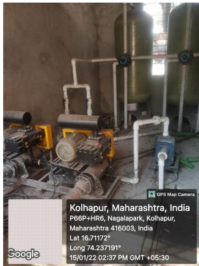
Picture 2. Wastewater treatment plant at Shrimati Sushiladevi Girls Hostel
