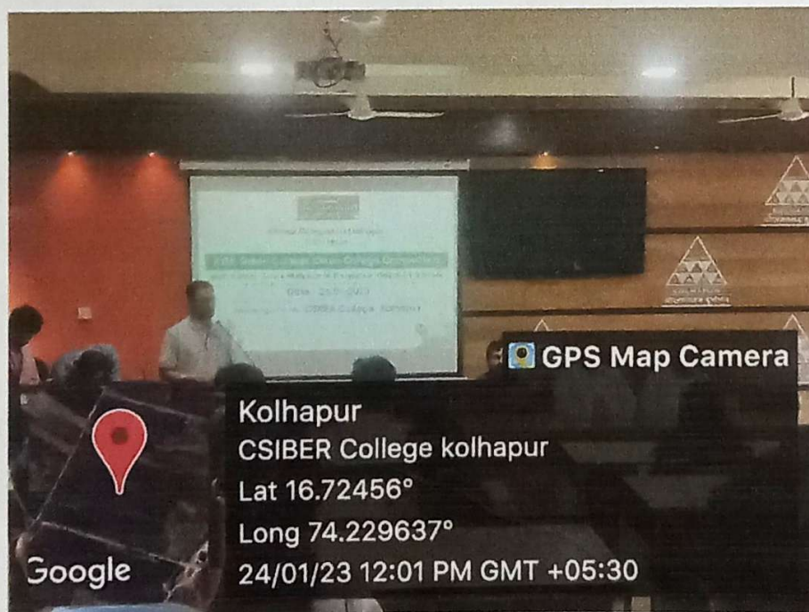
Inagural Function
